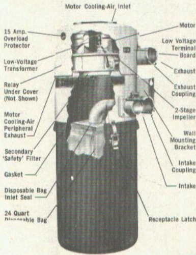
Model 350 — Power Unit
